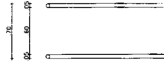
03 VISTA FRONTAL ESCALA 1/30
